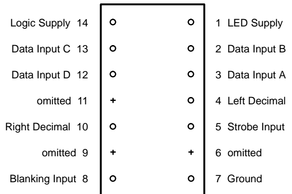
PACKAGE P 14-LEAD PDIP (BOTTOM VIEW)
